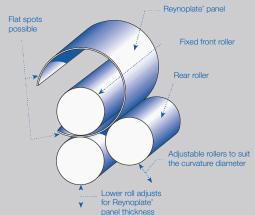
FIGURE 5 Roll Forming
