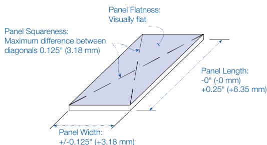
FIGURE 1 Manufacturing Tolerances
