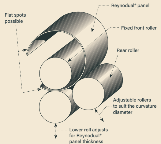
FIGURE 8 RADIUSING
