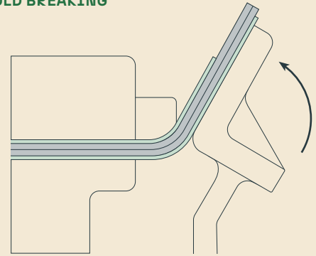
FIGURE 7 FOLD BREAKING
