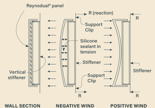
FIGURE 15 STIFFENER BEHAVIOR UNDER WIND LOAD
