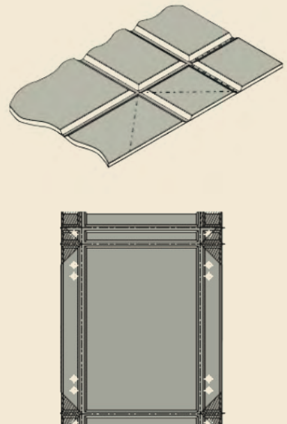
FIGURE 6 PANEL ROUTING & LAYOUT
