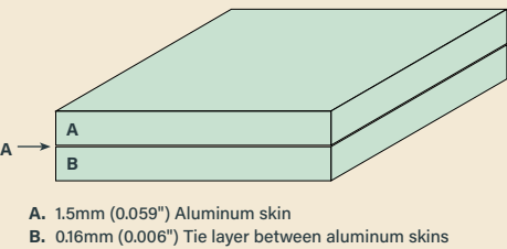
FIGURE 1 REYNODUAL® 3MM BONDED SHEET
