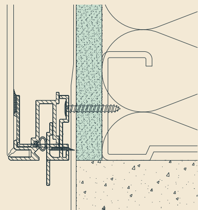
FIGURE 11 CAPTURED EDGE EXTRUSION
