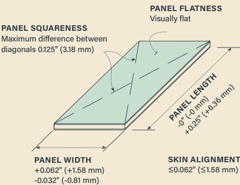
FIGURE 2 MANUFACTURING TOLERANCES
