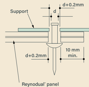
FIGURE 10 RIVETING WITH EXPANSION
