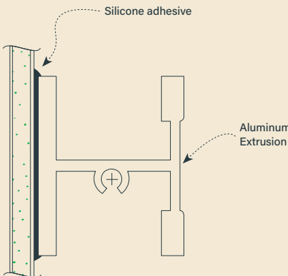
FIGURE 15 SECTION THRU STIFFENER
