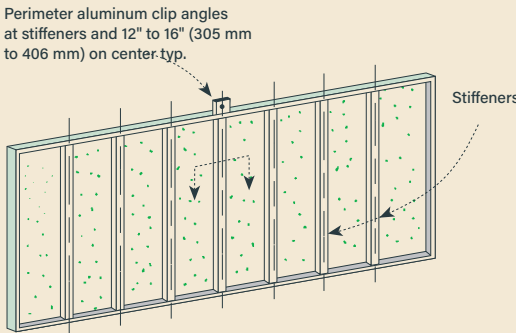
FIGURE 14 REAR VIEW OF STIFFENED ROUT & RETURN PANEL
